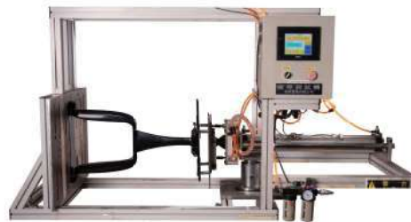
Cycle Testing Machine
